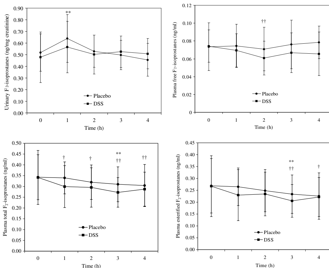
Fig. 1. Urinary and plasma F 2 -isoprostanes concentrations after placebo and dark soy sauce meal. Paired, two-tailed Student's t tests indicate **significance at p < 0.01 versus 0 h placebo; †significance at p < 0.05 and †† at p < 0.01 versus 0 h DSS.
